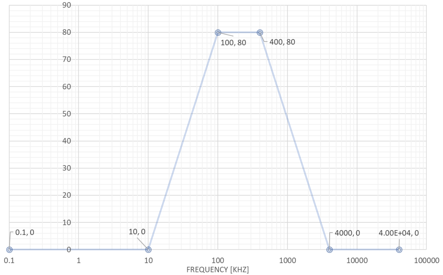
Figure 5 PROT6 chirp filter inline Minimum Differential Mode Attenuation
