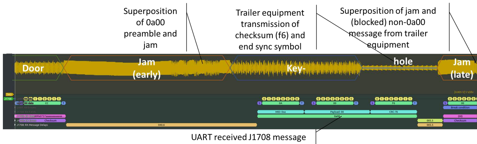
Figure 13 Description of a successful keyhole signal example
