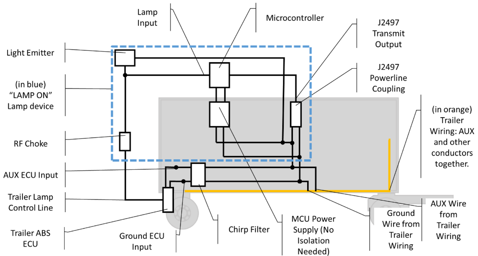
Figure 16 SOLNB LAMP detect circuit "LAMP ON" Lamp Device
