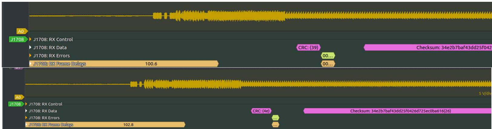
Figure 10 J2497 Receivers are more sensitive to corruption during the preamble phase
