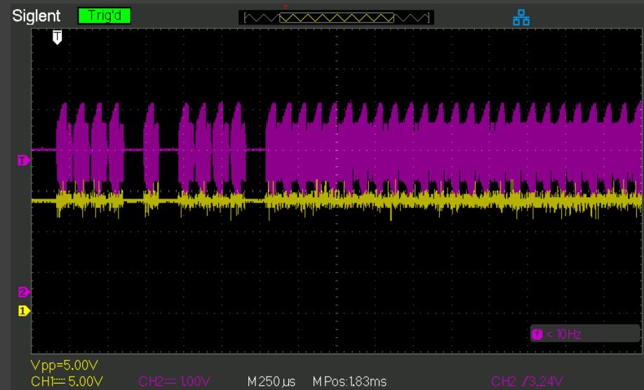
PWM result after receiver filtering (left: orange / right: purple)
